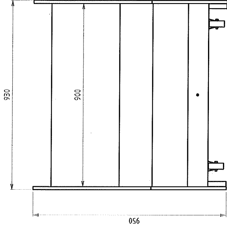
Vista Frontal
